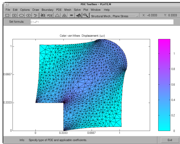
Visualization of the von Mises Effective Stress and the Displacements Using Deformed Mesh
